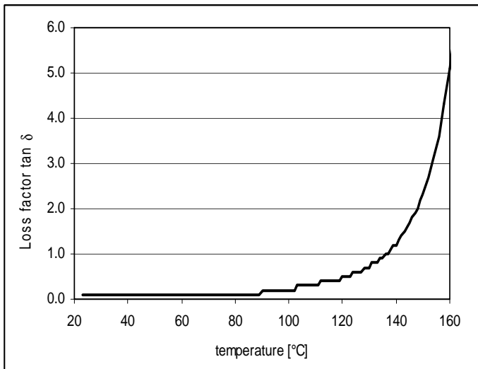
Figure 4: Loss factor (tan δ) at 50 Hz (IEC 60250)
